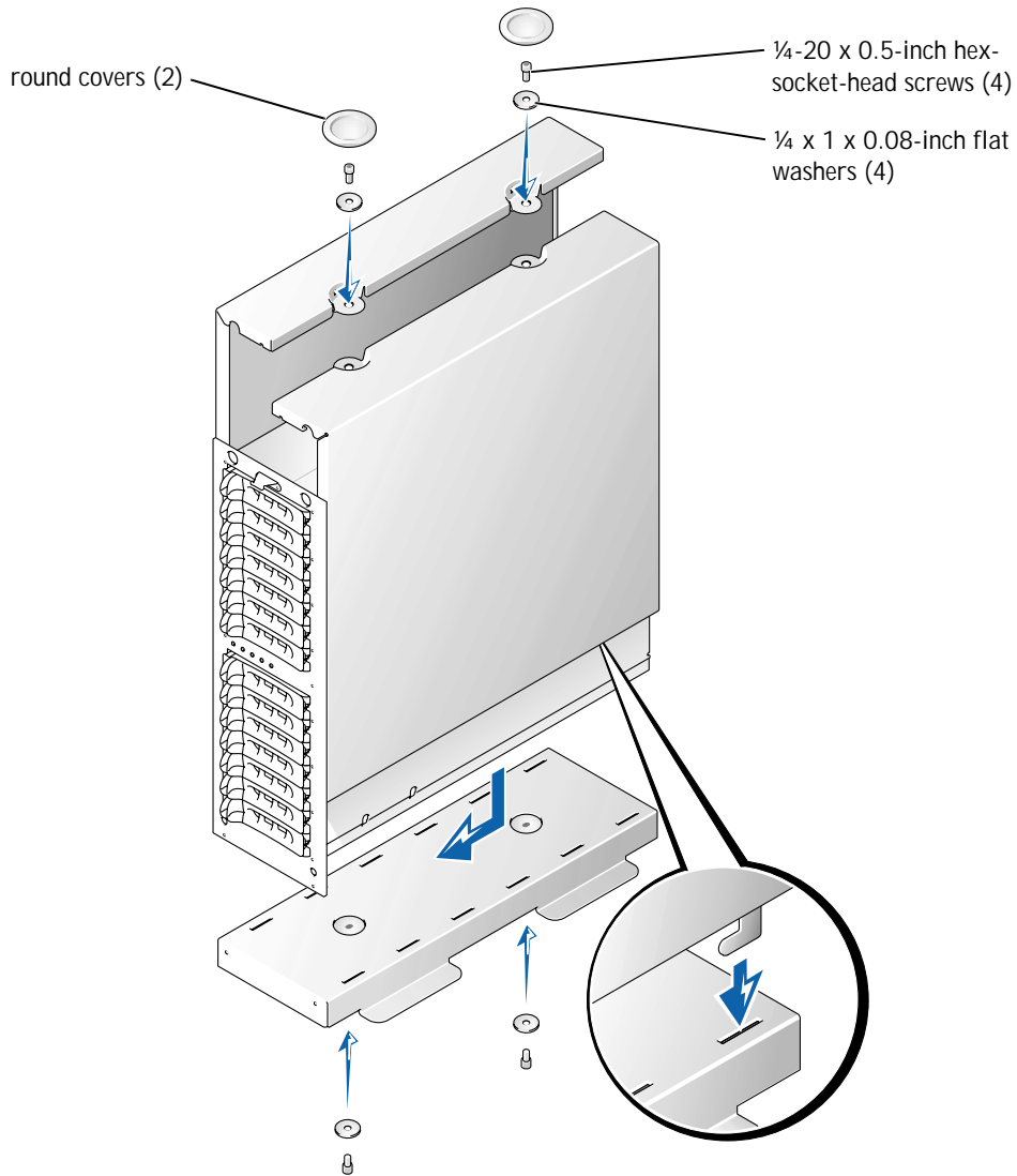
Figure 1-4. Installing the Tower System Cover
